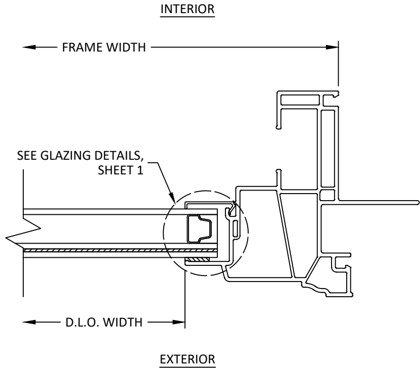
E 4 HORIZONTAL SECTION FIXED JAMB
