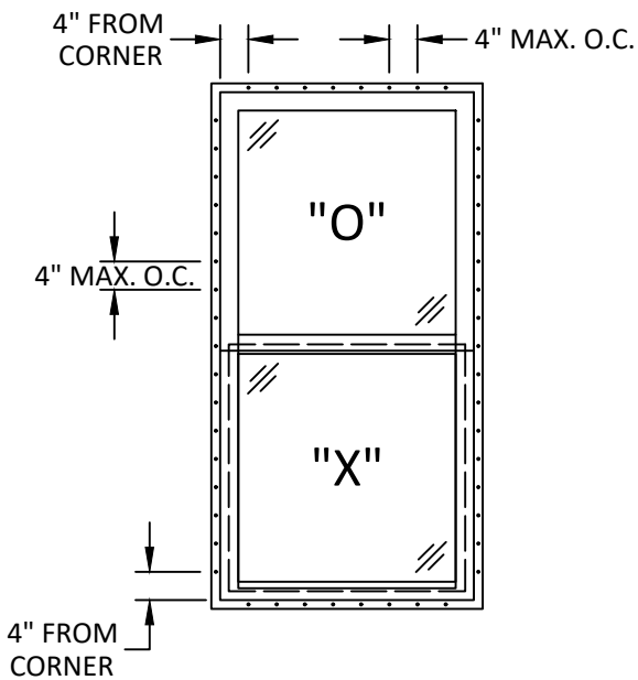
ANCHOR LAYOUT NAIL FIN
