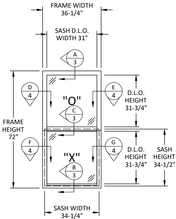
TYPICAL ELEVATION
