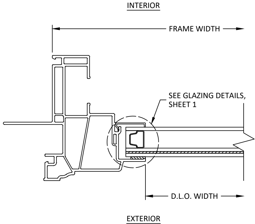
D 4 HORIZONTAL SECTION FIXED JAMB
